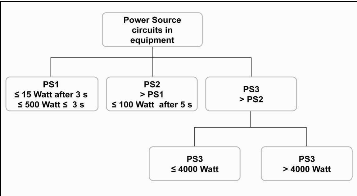
Figure 7: IEC62368 classifies three different power sources PS1, PS2 and PS3.
