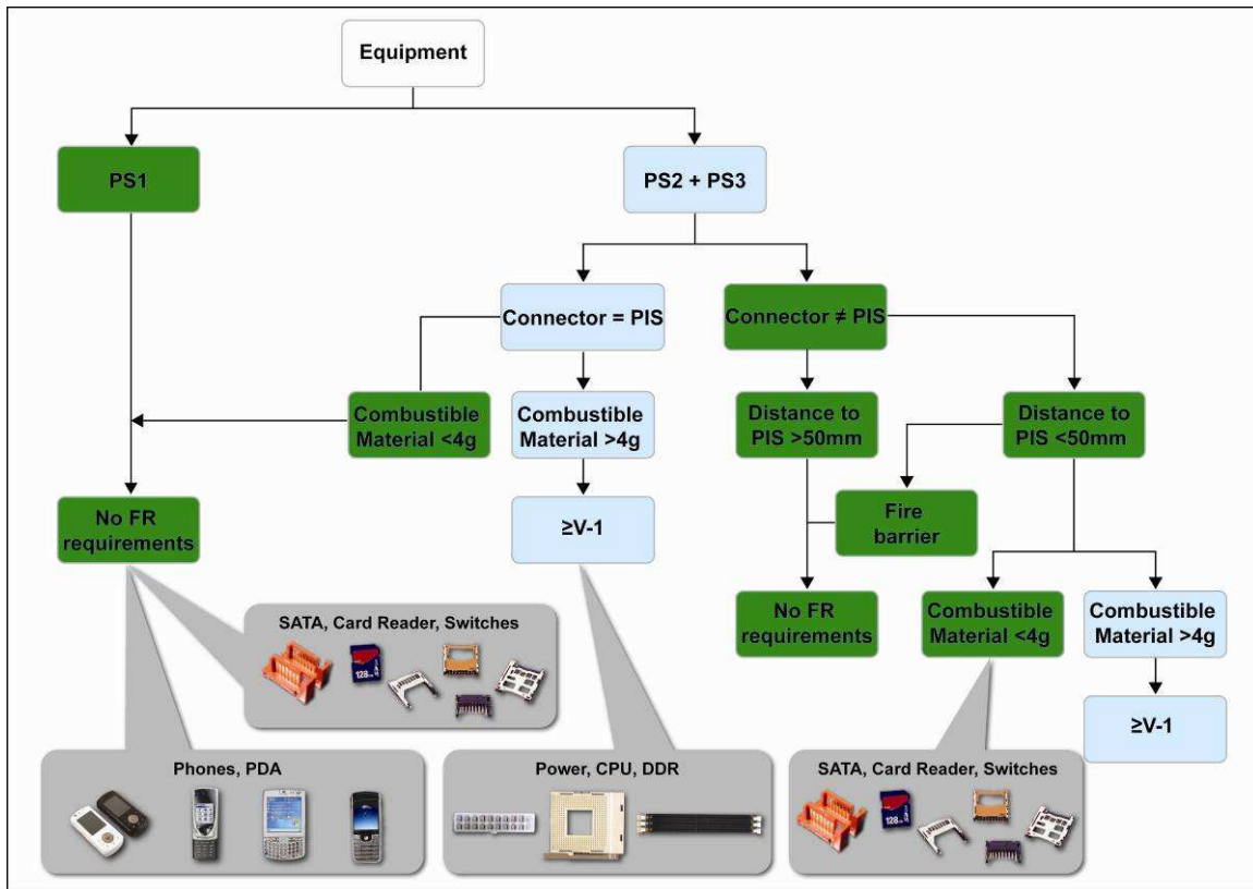
Figure 9: Prevent Ignition, internal connectors. Power level categorization and flame retardance requirements of internal connectors based on IEC62368 specification to prevent ignition. For illustration some connectors and applications are illustrated.
