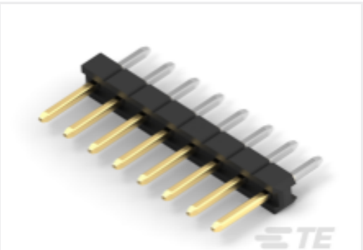
TE Part #2-2823088-5 25P,2MM,BRK HDR,SRVT,2.8,0.76AU, TB
