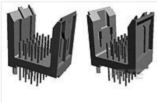
TE Part #5536514-1 2MMFB,ASY,024,SIG,HDR,EN,4.25
