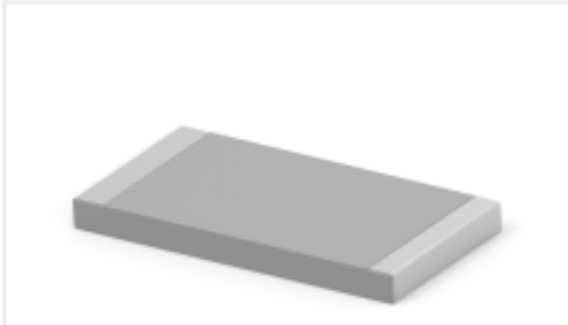
TE Part #5-2176331-1 CRGP 2512 150K 1%
