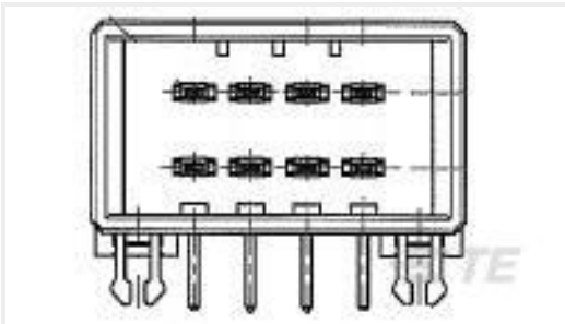
TE Part #1717412-2 DYNAMIC D-3100D H-HDR ASSY 8P PdNI & Au
