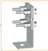
L5 Line Clamp to suit cables up to 1.38 in approximately 1250 kcmil
