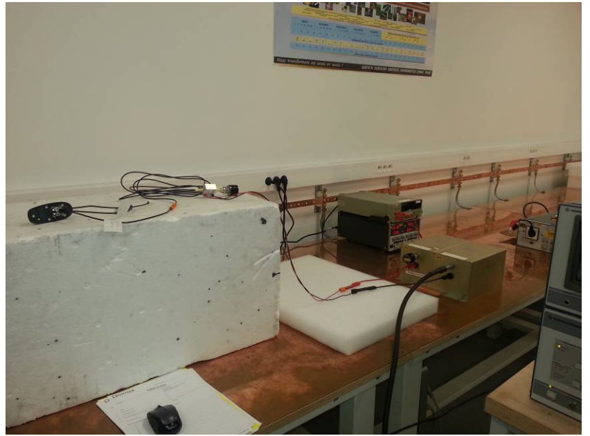
(Typical installation for conducted emissions)
