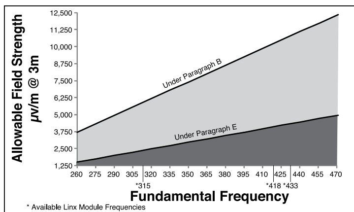
Figure 2: Allowed Output Power
