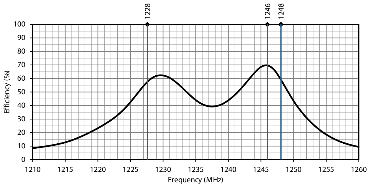
Figure 11. ANT-GNCP-TH25AL12 Antenna Radiation Efficiency, L2 Bands
