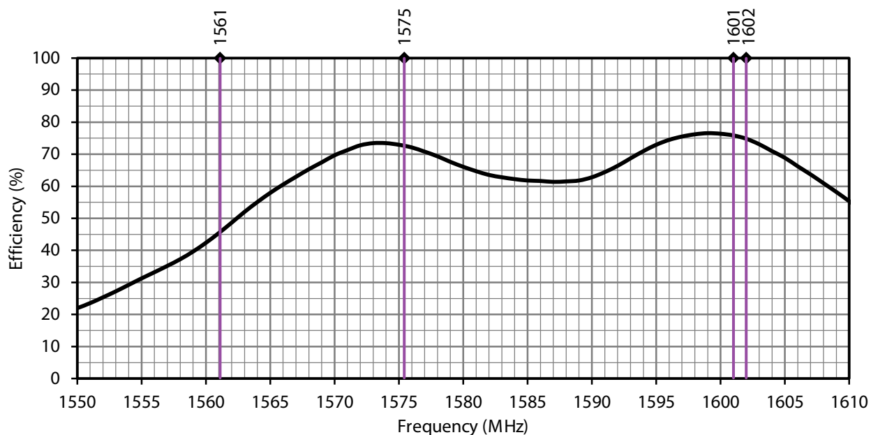
Figure 10. ANT-GNCP-TH25AL12 Antenna Radiation Efficiency, L1 Bands
