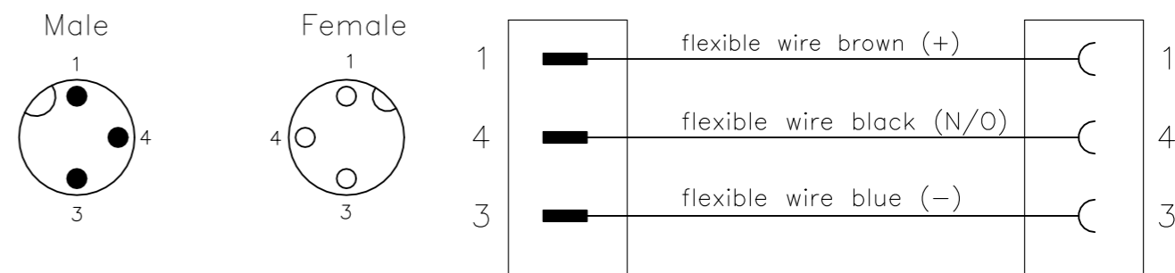
Contact Layout
