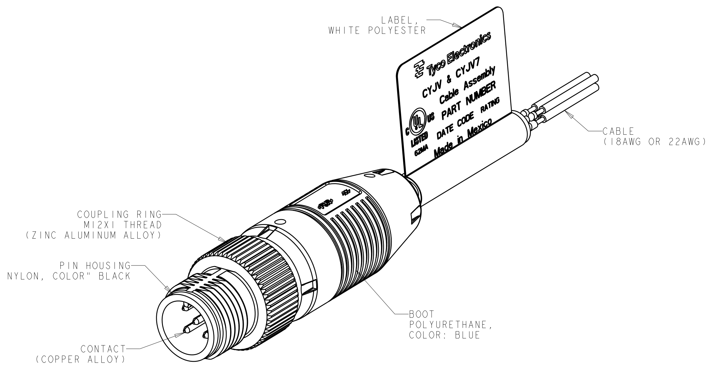
ISOMETRIC VIEW SCALE 3:1
