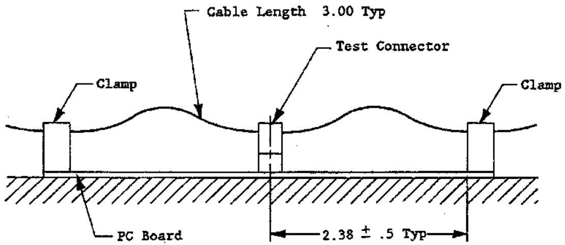
Figure 4 Vibration Fixture
