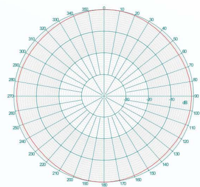
H Plane 5.5 GHz
