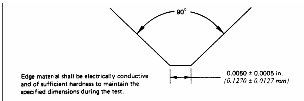
Figure 2. Dynamic Cut-Through Edge
