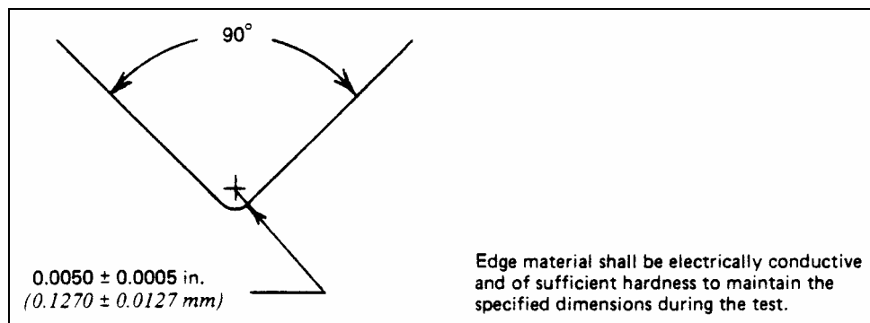
Figure 1. Scrape-Abrasion Edge
