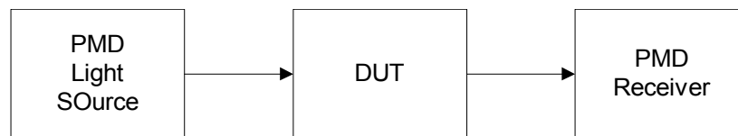
TP-910 Figure 4-121 Configuration for PMD Tests (not from GR-910)
