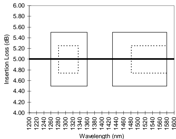
GR-910 Figure 5-5 3 dB Attenuator Optical Bandpass Spectra
