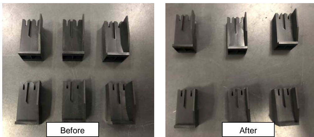
Figure 3- typical specimens following mold stress test
