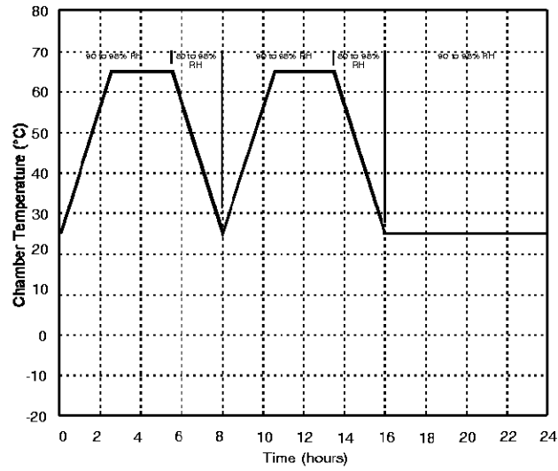
Figure 3 Typical Humidity-Temperature Cycling Profile
