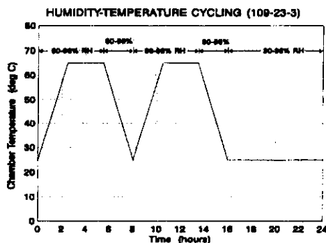
Figure 3 Typical Humidity-Temperature Cycling Profile
