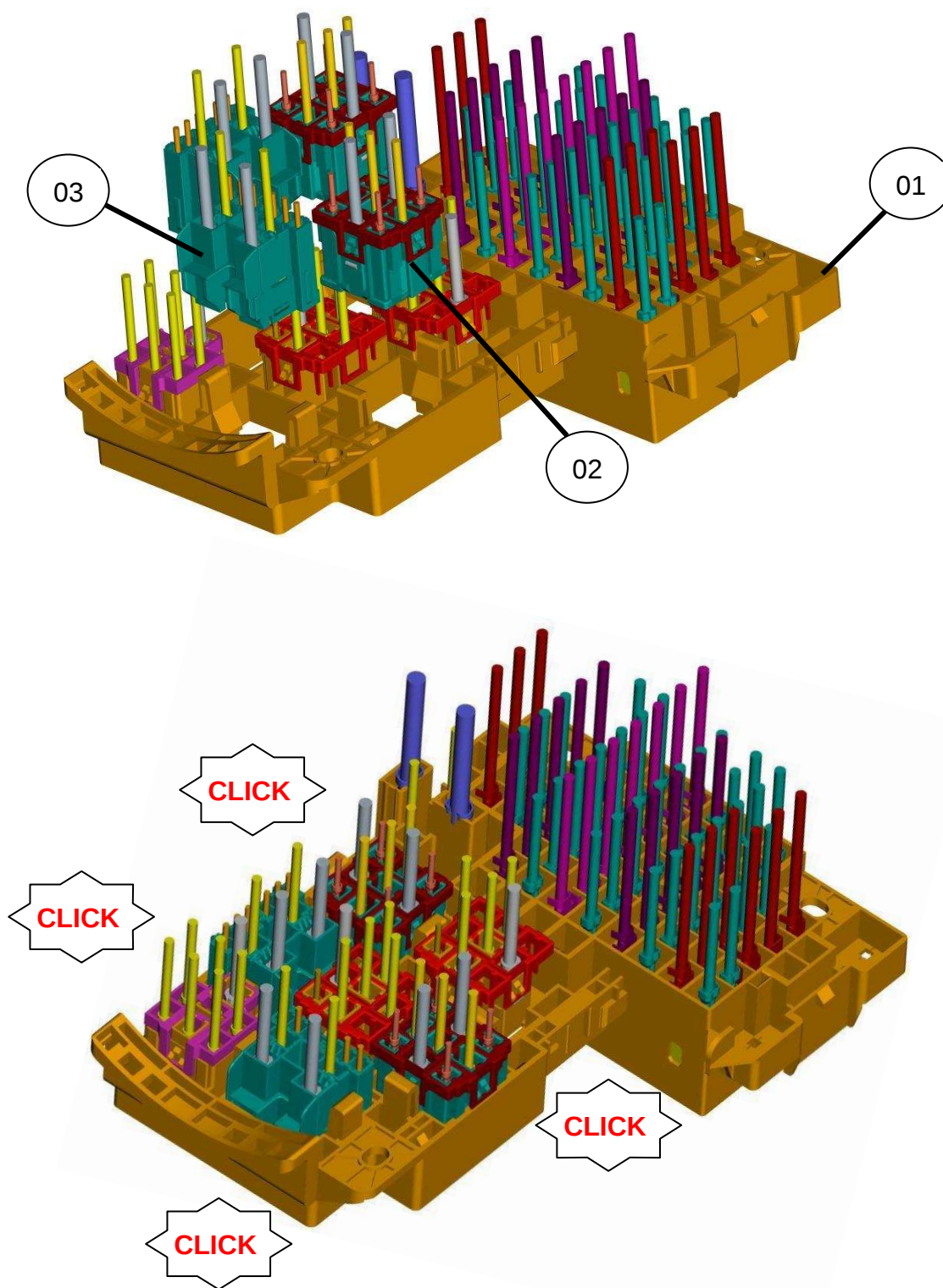
FUSE BOX ASSEMBLY – PN T/E 1380007-1
