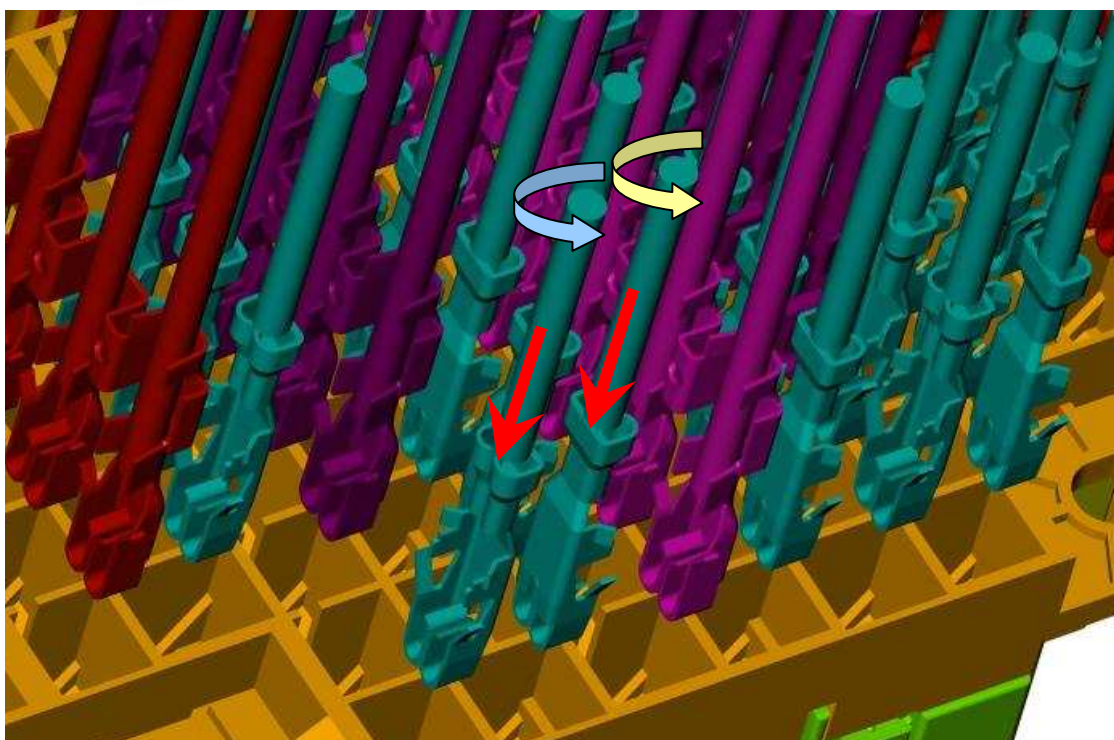
Detail "A"
