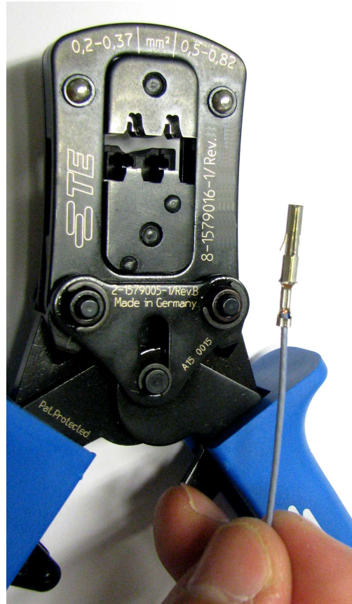
Picture 9: Checking the crimping contact
