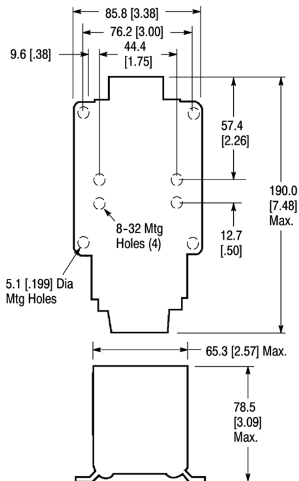
Model 7032 (Mounting Dimensions)
