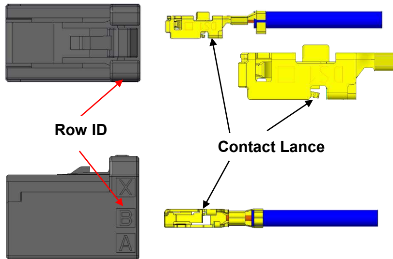
Figure.5 Insertion direction of Receptacle Contact
