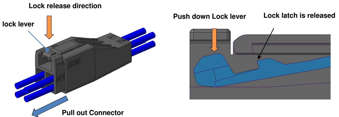
Figure.8 Un-Mating connector
