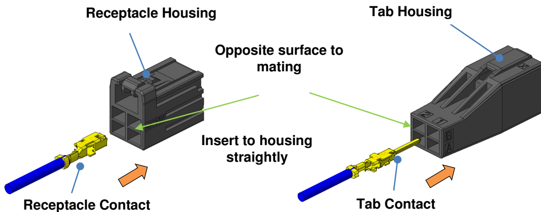
Figure.6 Contact Insertion
