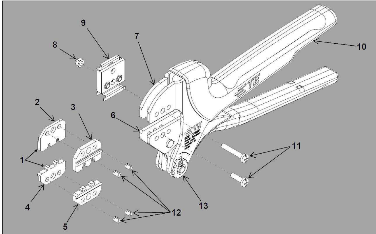
Figure 1: SDE Crimp Commercial Hand Tool Assembly 2063537-1 with Die Assembly 2063537-2
