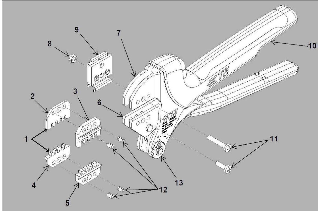
Figure 1: SDE Crimp Commercial Hand Tool Assembly 2063536-1 with Die Assembly 2063536-2
