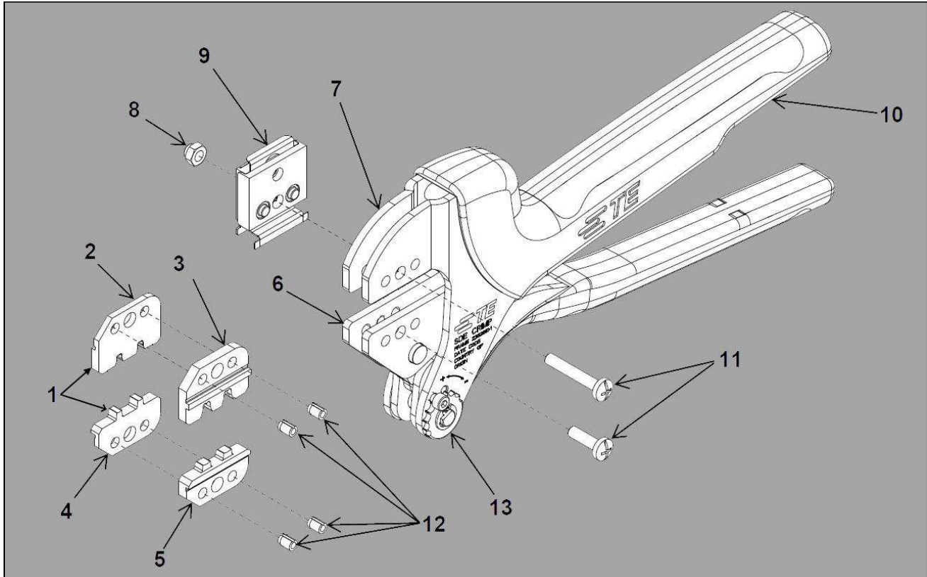
Figure 1: SDE Crimp Commercial Hand Tool Assembly 2063379-1 with Die Assembly 2063379-2
