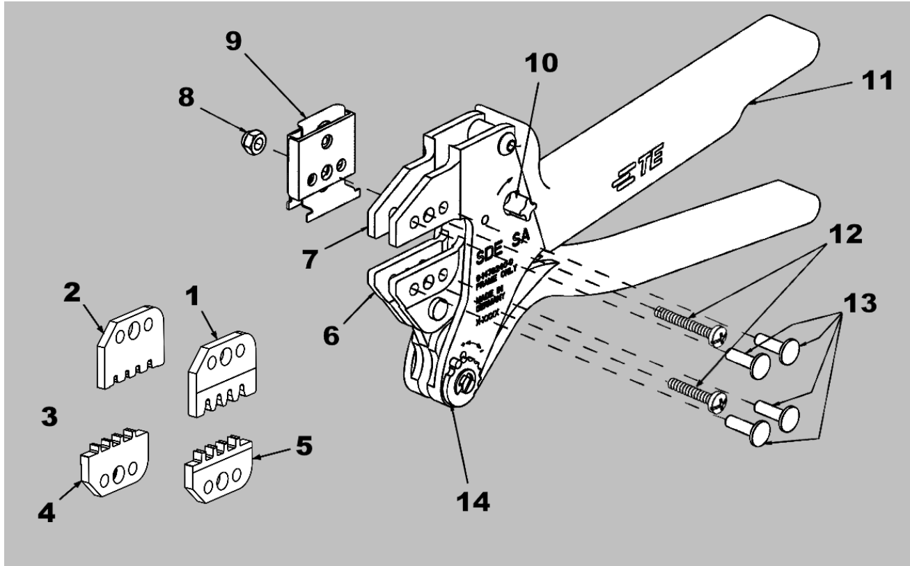
Figure 1: SDE-SA Commercial Hand Tool Assembly 2379969-1 with Die Assembly 2379969-2
