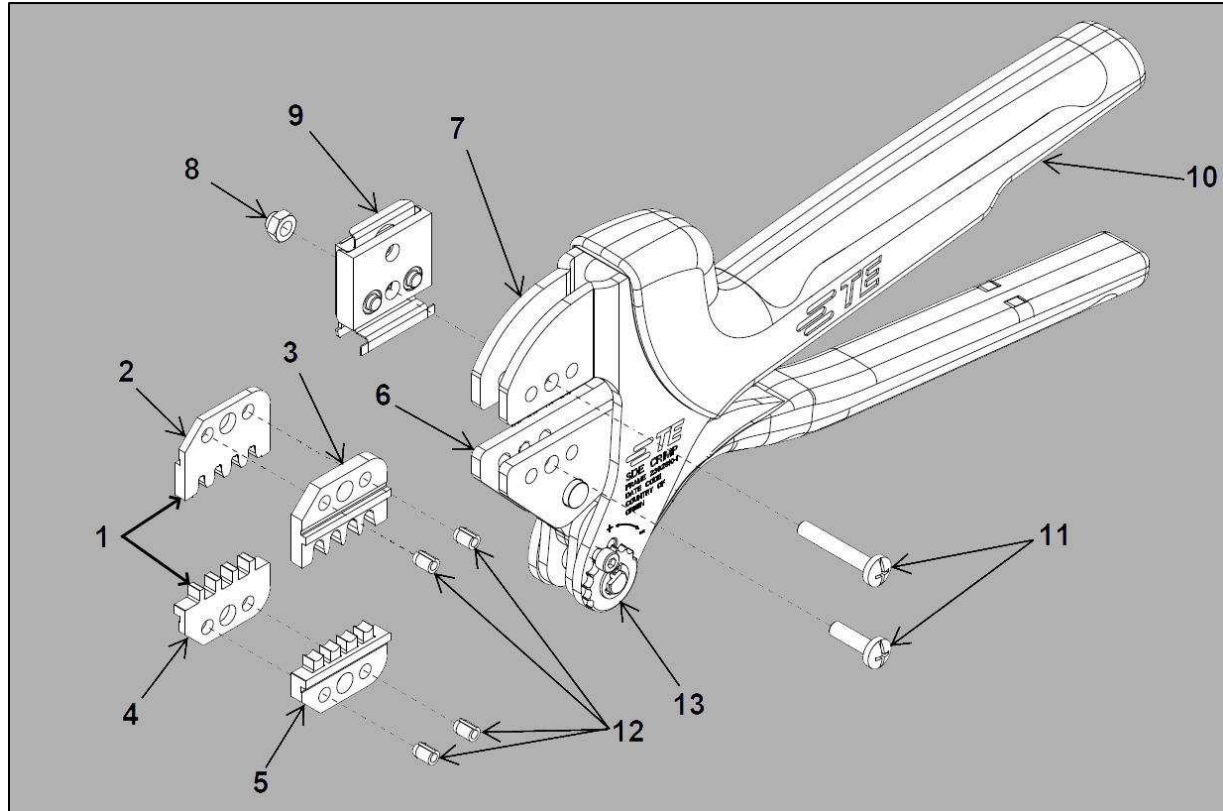
Figure 1: SDE Crimp Commercial Hand Tool Assembly 2031676-1 with Die Assembly 2031676-2
