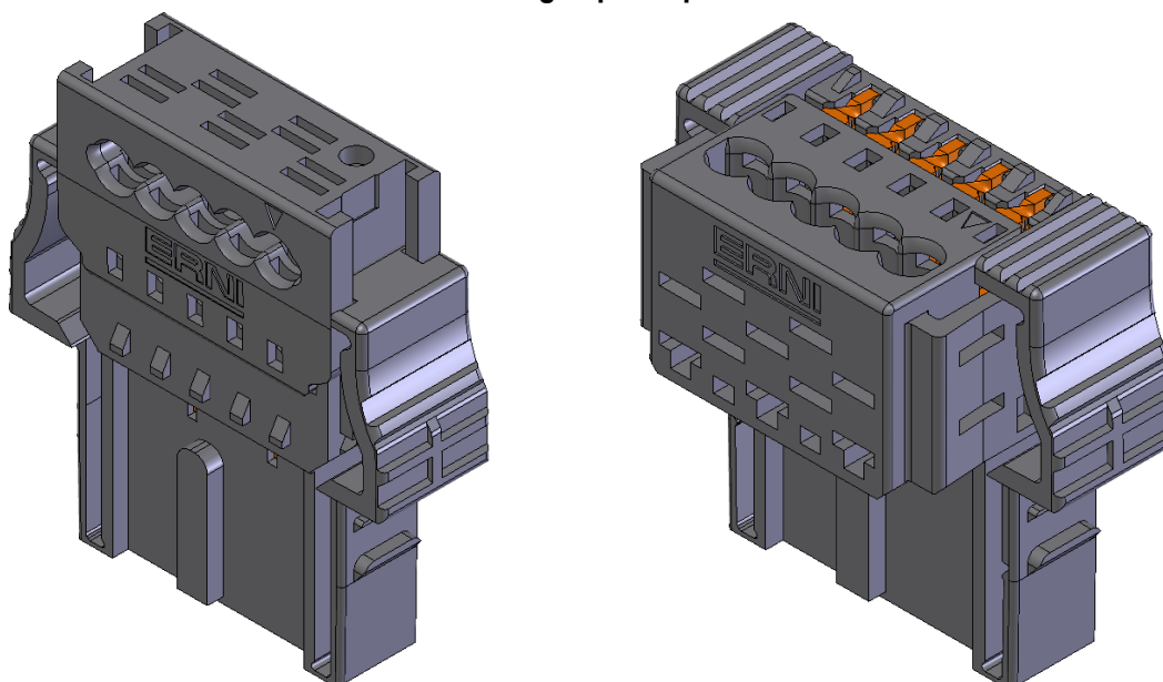
Figure 1 90° cable outlet (e.g. 524431-E, closed) 180° cable outlet (e.g. 504958-E, pre-assembled)
