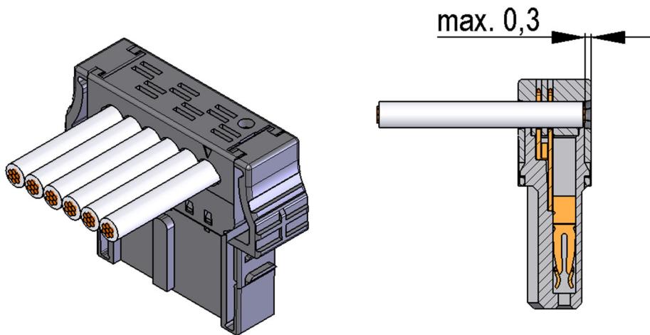
Figure 4 Undercut
