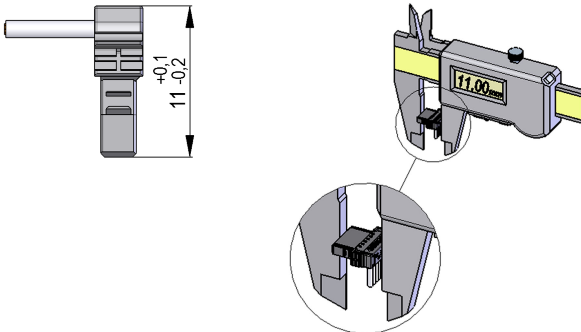
Figure 16 90° cable outlet
