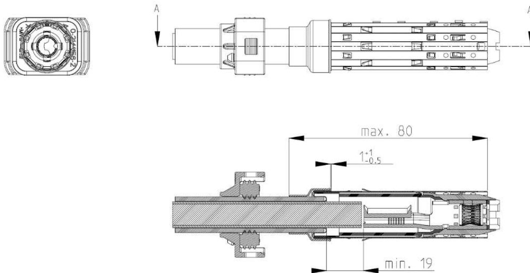
Figure 11: Cable assembly/Kabelbaugruppe
