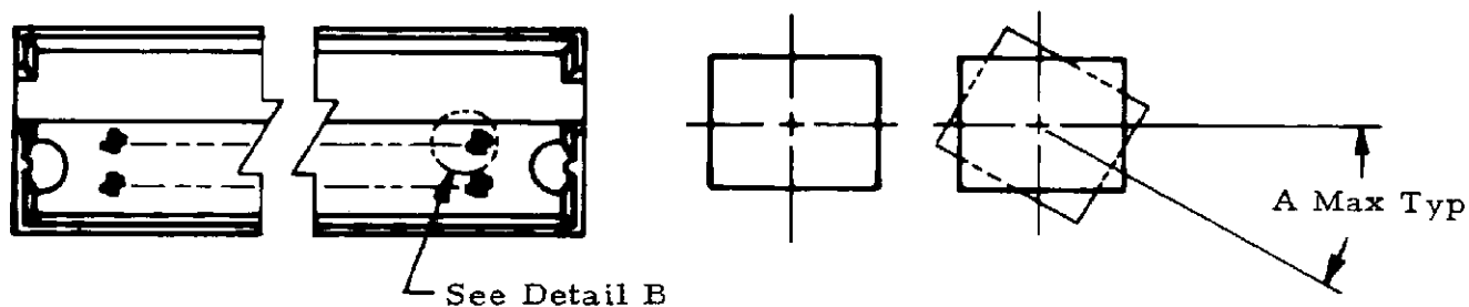
Detail B
