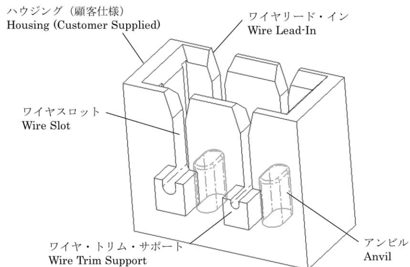
B. Housing
