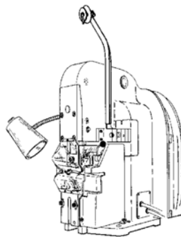
AMP-TAPETRONIC Machine 69875 (409-1993)
