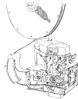
AMP-O-ELECTRIC Model "G" Terminating Machine 354500-[] (409-5842)
