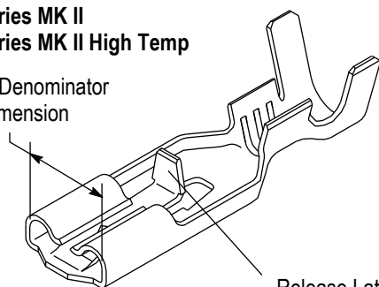
Release Latch
