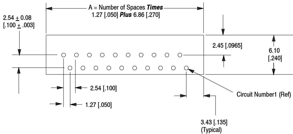
Layout for Connectors with Centerlines on 1.27 [0.050]
