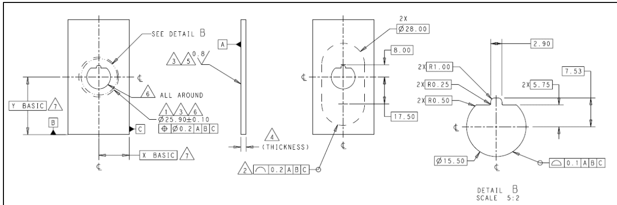
Figure 28: Alternative recommended panel/enclosure geometry for header 2325102-1.
