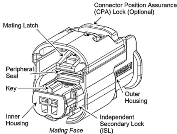
2 Position enetSEAL+ Plug Assembly
