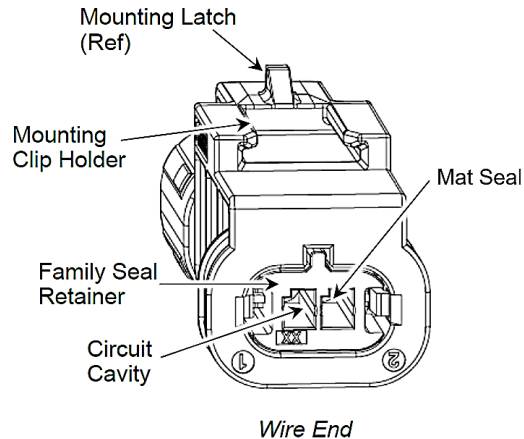
2 Position enetSEAL+ Cap Assembly
