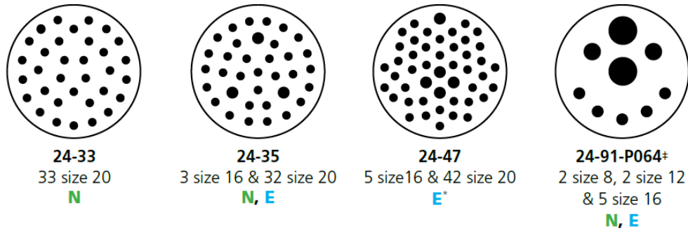
Figure 3 Pin Arrangements
