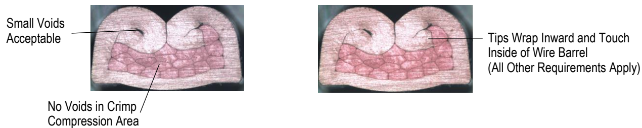
Unacceptable Wire Barrel Crimp
