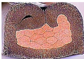
Uneven Crimp and Wall Thickness
