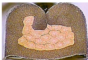
Uneven Crimp and Wall Thickness and Flash on Both Sides
