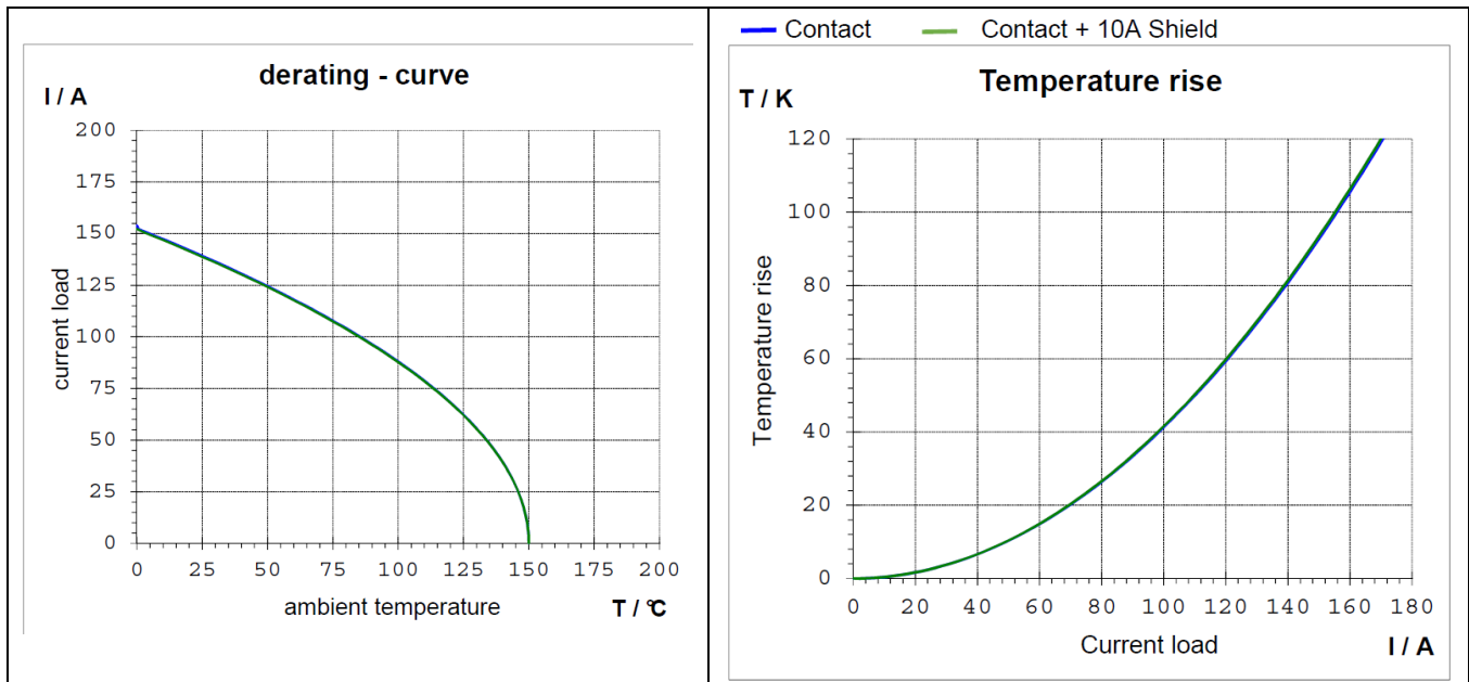
Figure 2: Derating and temperature rise in housing. Current loaded on contacts + 10A on shield according LV215-2
