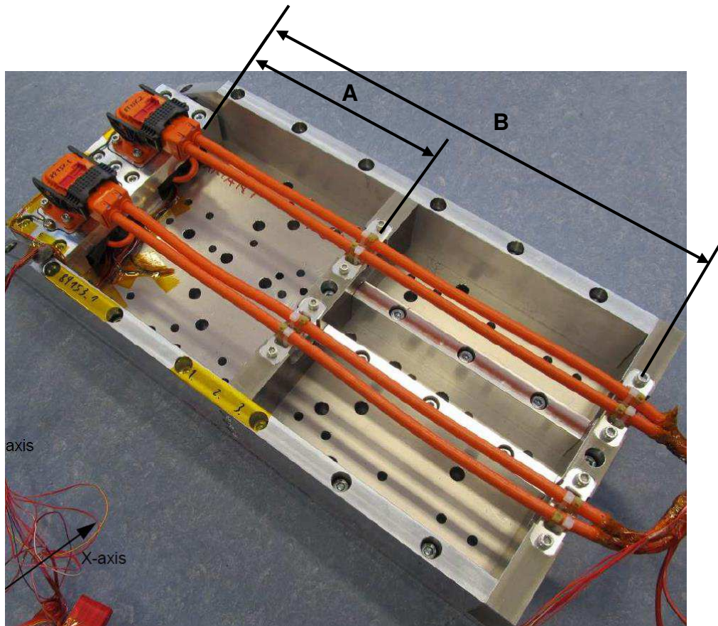
Figure 3: Connector on vibration device
