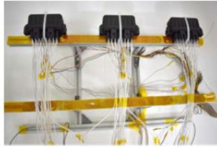
Test setup
