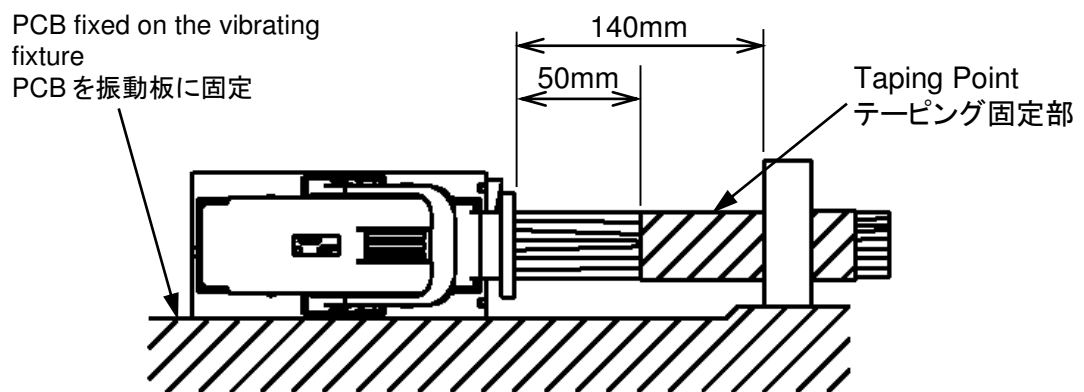
Fig.10 Vibration Test Condition 振動試験の固定状態
