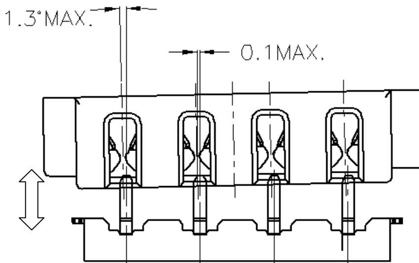
Fig.4-2 傾き許容量(耐久性試験) Fig.4-2 Tilt allowance for durability test
