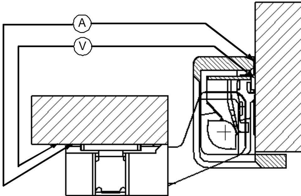
Fig.2 総合抵抗測定点 Fig.2 Termination Resistance Measuring Points
