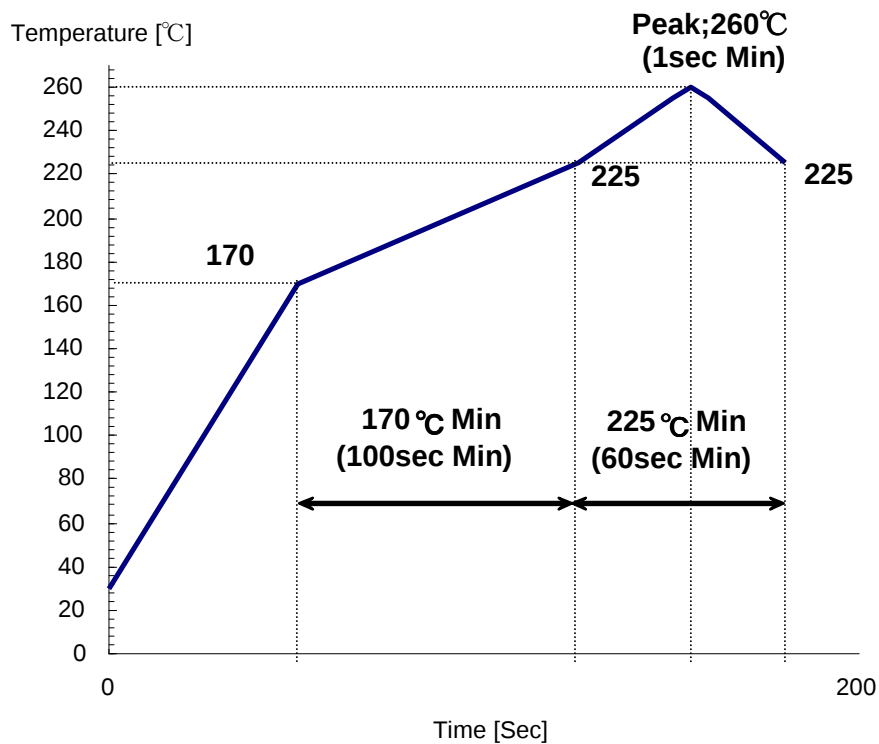
Fig.6 Reflow Profile
