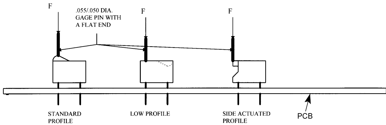
Figure 4 Actuation Force
