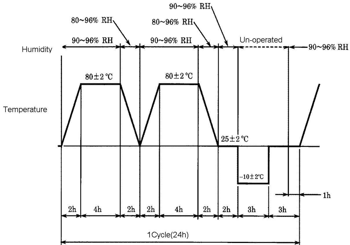
Fig. 9 Humidity-Temperature Cycling
