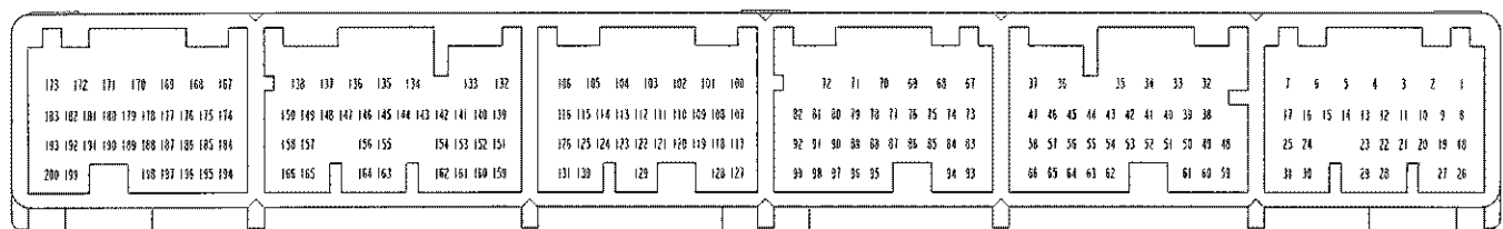
Fig.14 200 Position Circuit Layout
