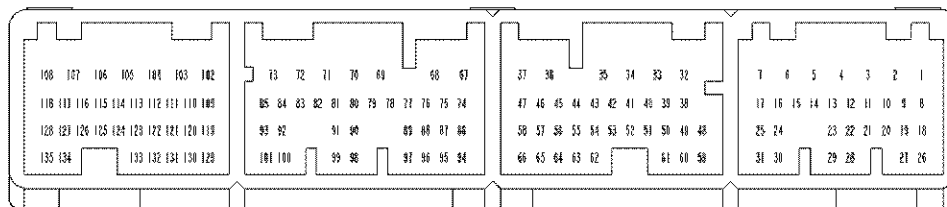
Fig.12 135 Position Circuit Layout
