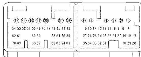
Fig.11 70 Position Circuit Layout
