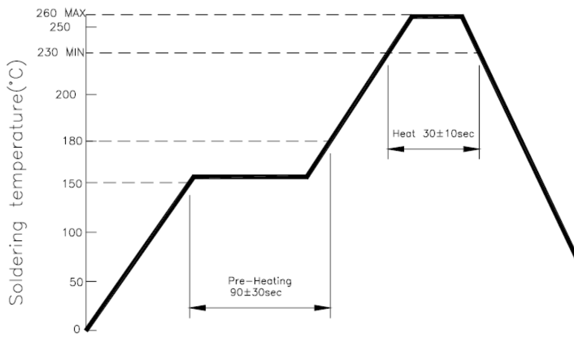
Temperature Profile of Reflow Soldering
