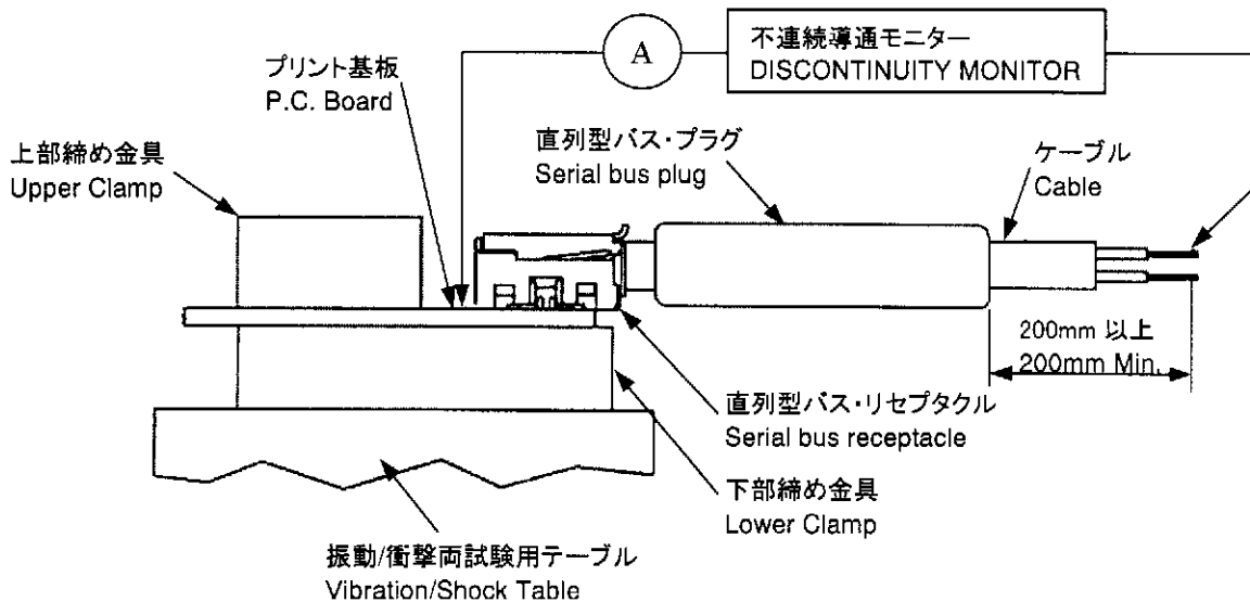
Fig.4 振動/衝撃両試験用取付け治具 Fig.4 Vibration & Physical Shock Mounting Fixture
