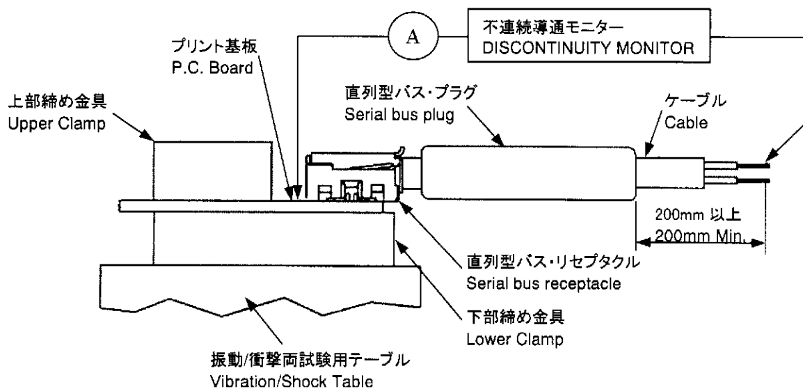
Fig.4 振動/衝撃両試験用取付け治具 Fig.4 Vibration & Physical Shock Mounting Fixture
