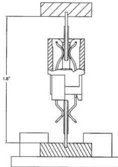
Figure 3 Vibration & Mechanical Shock Mounting Fixture
