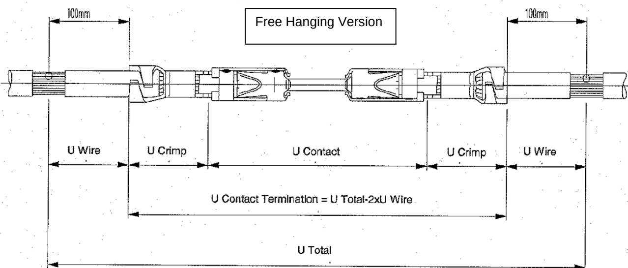
PCB MOUNTED CONNECTOR LLCR Measurement Points Figure BUSS BAR CONNECTOR LLCR Measurement Points Figure
