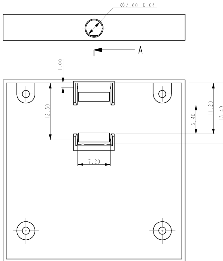
Figure 5 Test Cover for bending strength test
