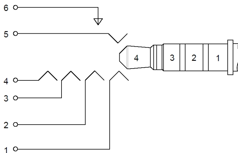
Figure 1. Connector side circuit diagram
