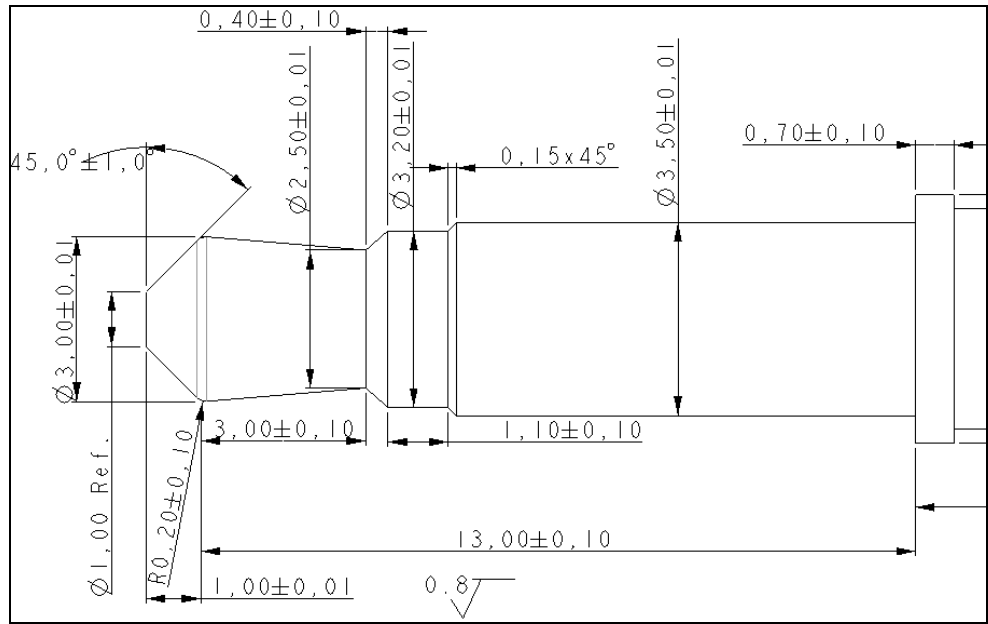
Figure 4. Test gauge
